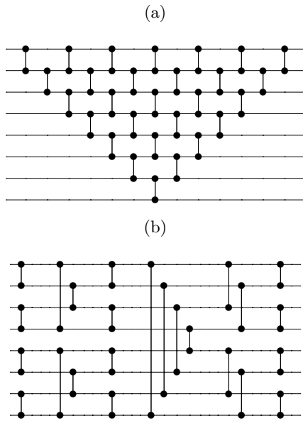
FIG. 2. Two examples of sorting networks on 8 inputs: (a) the insertion sort over a 1D nearest neighbour graph which sorts in time T = 2n - 3 , and (b) the bitonic sort over the hypercube that requires time T = \frac{1}{2} \log n(\log n + 1) .
