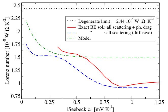
FIG. 10. Lorenz number L as a function of Seebeck coefficient S at T = 300 K. The red solid line (dashed blue line) is from the solution of the BE with (without) the phonon drag. The green dot-dashed line the model proposed in Ref. 48. The black dotted horizontal line is the Wiedemann-Franz result.
