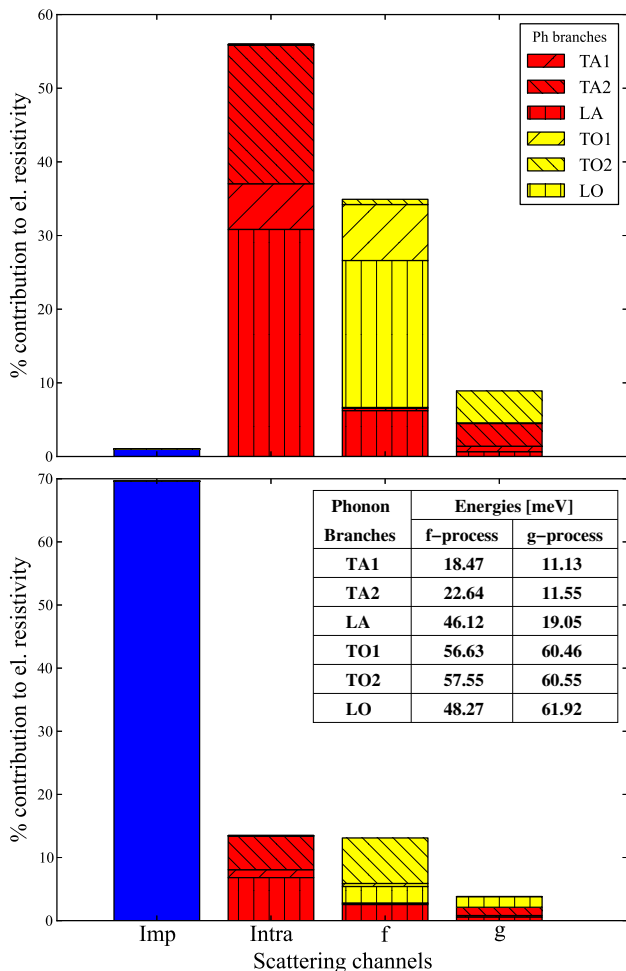
FIG. 4. Relative contribution of the different scattering mechanisms to electrical resistivity at T = 300 K. Carriers' concentrations are 2.4 \times 10^{14} \text{cm}^{-3} (upper panel) and 1.3 \times 10^{19} \text{cm}^{-3} (lower panel). The charged impurities' contribution (Imp), intra-valley phonon scattering (Intra) and inter-valley phonon scattering (f and g stand for f-processes and g-processes, described in Ref. 20) are shown. The phonon scattering are separated in acoustic (dark red) and optical (light yellow) branches, and different patterns are used for the modes: diagonal lines for TA1 and TO1, dense diagonal lines for TA2 and TO2 and vertical lines for LA and LO. The phonon energies of the different modes are also shown.
