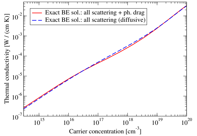
FIG. 8. Electronic thermal conductivity as a function of carrier concentration at T = 300\text{K} . The red solid line is from the solution of the BE that includes all the scattering mechanisms and the phonon drag. The blue long-dashed line is the same as the red solid line but without the phonon drag.
