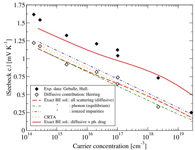
FIG. 5. Seebeck coefficient as a function of carrier concentration at T = 300 K. The solid red line is the total Seebeck coefficient, the red dashed line is the diffusive contribution, the orange dotted line is the CRTA result, the green dot-dash-dashed (blue dot-dot-dashed) line is the diffusive S computed including only phonon (impurity) scattering. The solid black diamonds are the experimental results, 14 while the open diamonds represent the diffusive Seebeck extracted from the experimental data. 14,15
